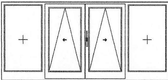
Type C 2 tilt and slide, 2 fixed
