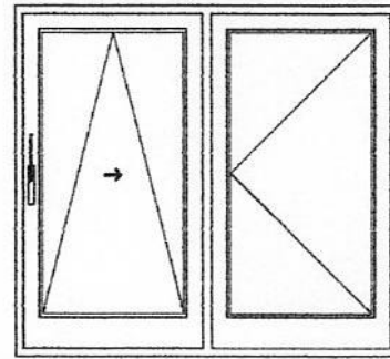
Type A 1 tilt and slide, 1 balanced sash or tilt and turn
